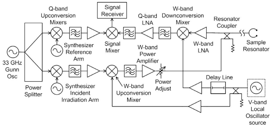
Fig. 3. Frequency-swept W-band EPR bridge functional schematic. See Fig. 2 for components key. Nominally, the incident irradiation arm synthesizer is set to 2 GHz, and the reference arm synthesizer is set to 3 GHz. 33 GHz is upconverted to 35 GHz and then to 94 GHz. The EPR signal at 94 GHz is downconverted to 35 GHz and then to 1 GHz at the signal mixer output.
