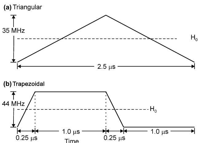
Fig. 1. Frequency-sweep waveforms: (a) example display of one of the triangular frequency-sweep waveforms used and (b) the trapezoidal waveform used for the data acquisition in Figs. 7 and 8. The H_0 lines show the position of the EPR line center in the frequency-sweep range.
