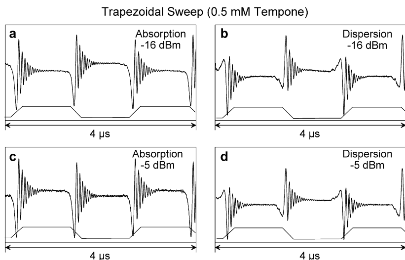
Fig. 7. Representative trapezoidal sweep responses for 0.5 mM TEMPONE obtained from using the waveform shown in Fig. 1b centered on the low field line. Sweep rates are 0.176 MHz/ns (equivalent to 3.8 kT/s). Fig. 7a and c as shown are double-baseline corrected as described in the text.
