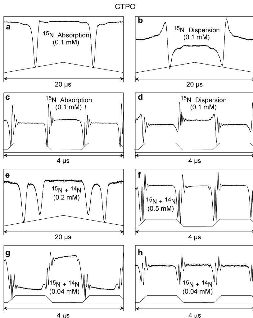
Fig. 8. Representative swept-frequency responses for the CTPO samples. Fig. 8a and b used 50 kHz triangular waveforms of 44.7 MHz deviation centered on the low field line. Fig. 8e used 50 kHz triangular waveforms of 45.3 MHz deviation centered between the two low field lines of ^{14}\text{N} + ^{15}\text{N} CTPO. Fig. 8c, d, f, g, and h used the trapezoidal waveform of 36.7 MHz deviation centered on the low field or between the two low field lines of the ^{14}\text{N} + ^{15}\text{N} CTPO. Sweep rates are 0.147 MHz/ns (equivalent to 5.25 kT/s). Fig. 8c and h are double-baseline corrected.
