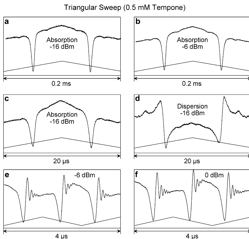
Fig. 6. Representative triangular-sweep spectral responses for 0.5 mM TEMPONE. Sweep profiles are indicated at the bottom of each display. Fig. 6a and b used 5 kHz waveforms of 35 MHz frequency deviation centered on the low field line. Fig. 6c and d used 50 kHz waveforms of 32 MHz deviation centered on the high field line, and Fig. 6e and f used 400 kHz waveforms of 25 MHz deviation centered on the low field line.
