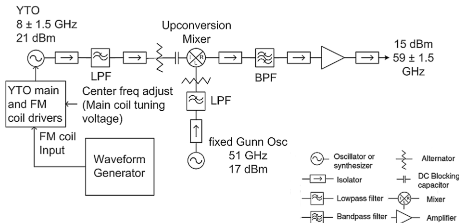
Fig. 2. V-band source: YIG-tuned oscillator (YTO) translated by a fixed frequency Gunn diode oscillator (Gunn Osc). LPFs isolate the mixer from oscillator harmonics. The BPF passes the upper sideband from the mixer.
