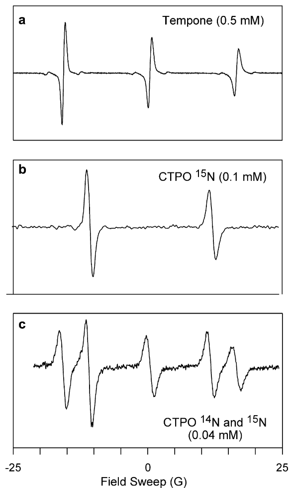
Fig. 5. W-band room temperature spectra of aqueous samples used in this study. Detailed information on sample preparation and resonator configuration are given in Refs. [3,6].
