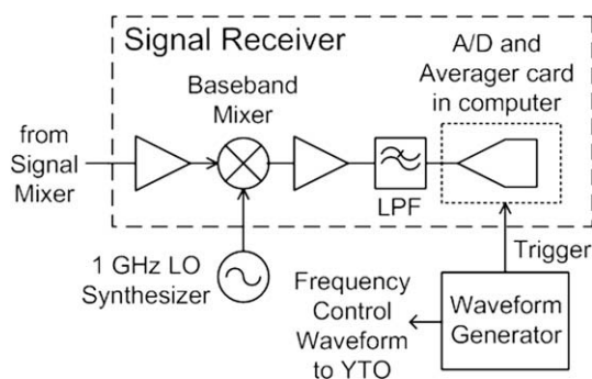
Fig. 4. Signal receiver detail. The 1 GHz LO synthesizer phase is adjusted for absorption or dispersion. The waveform generator synchronizes data collection with the frequency-sweep waveform.
